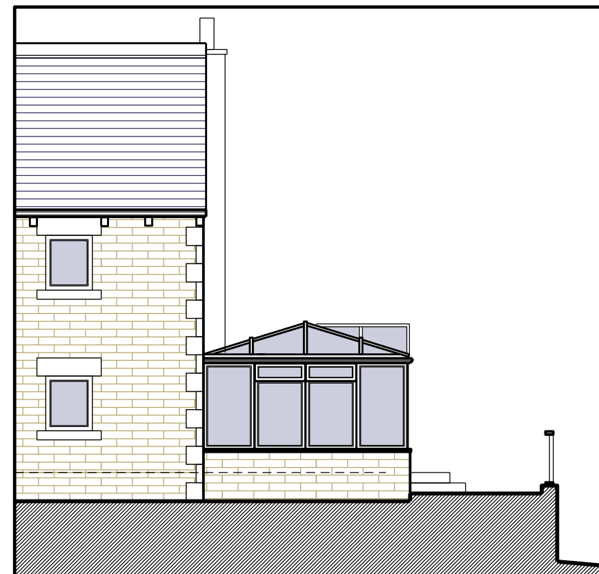
West Elevation
