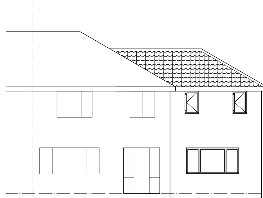
FRONT ELEVATION
