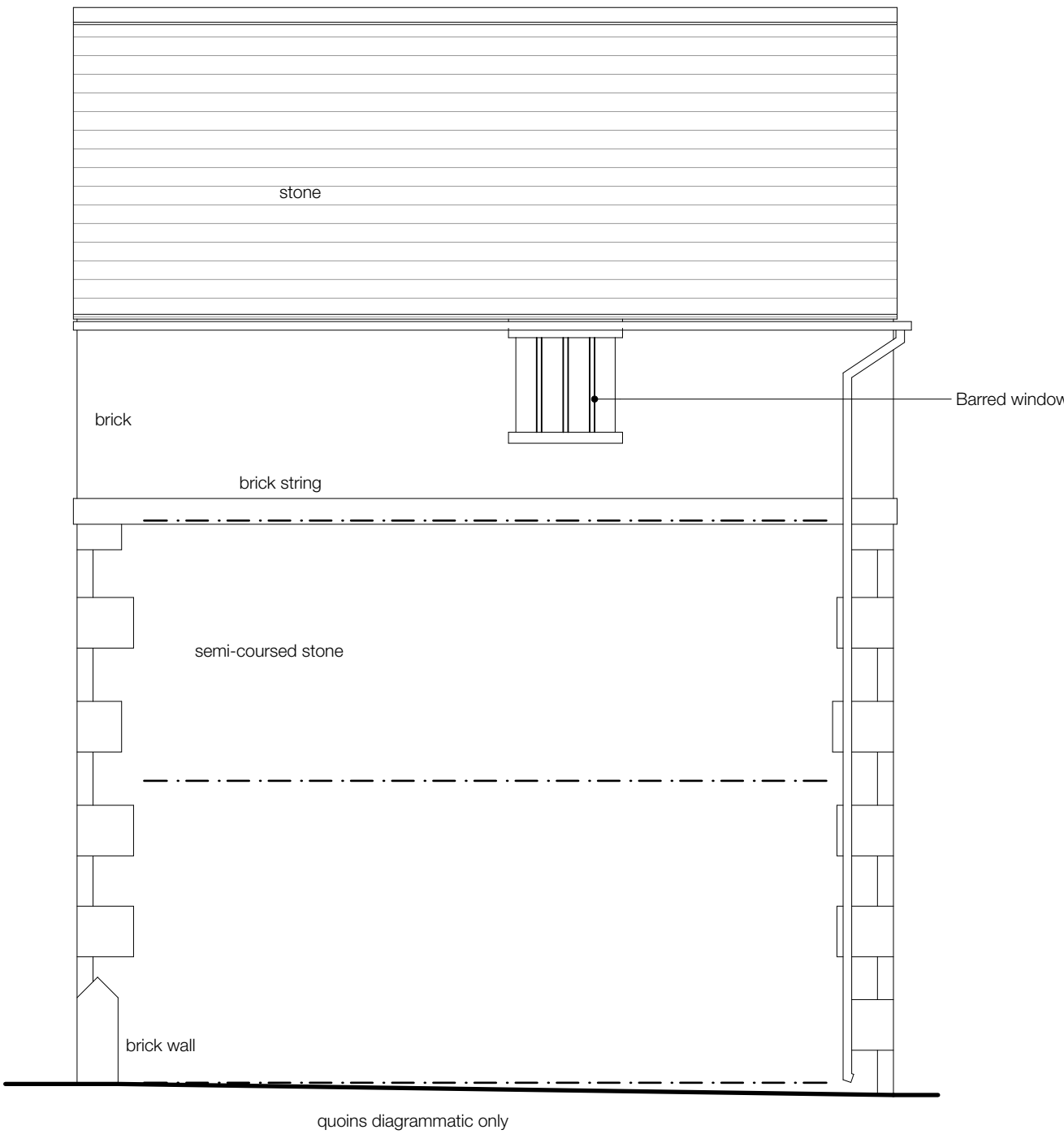
East Elevation (Existing)
