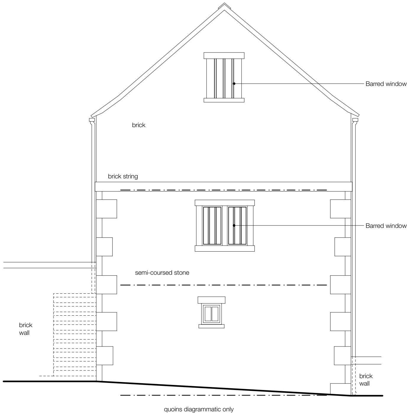
South Elevation (Existing)
