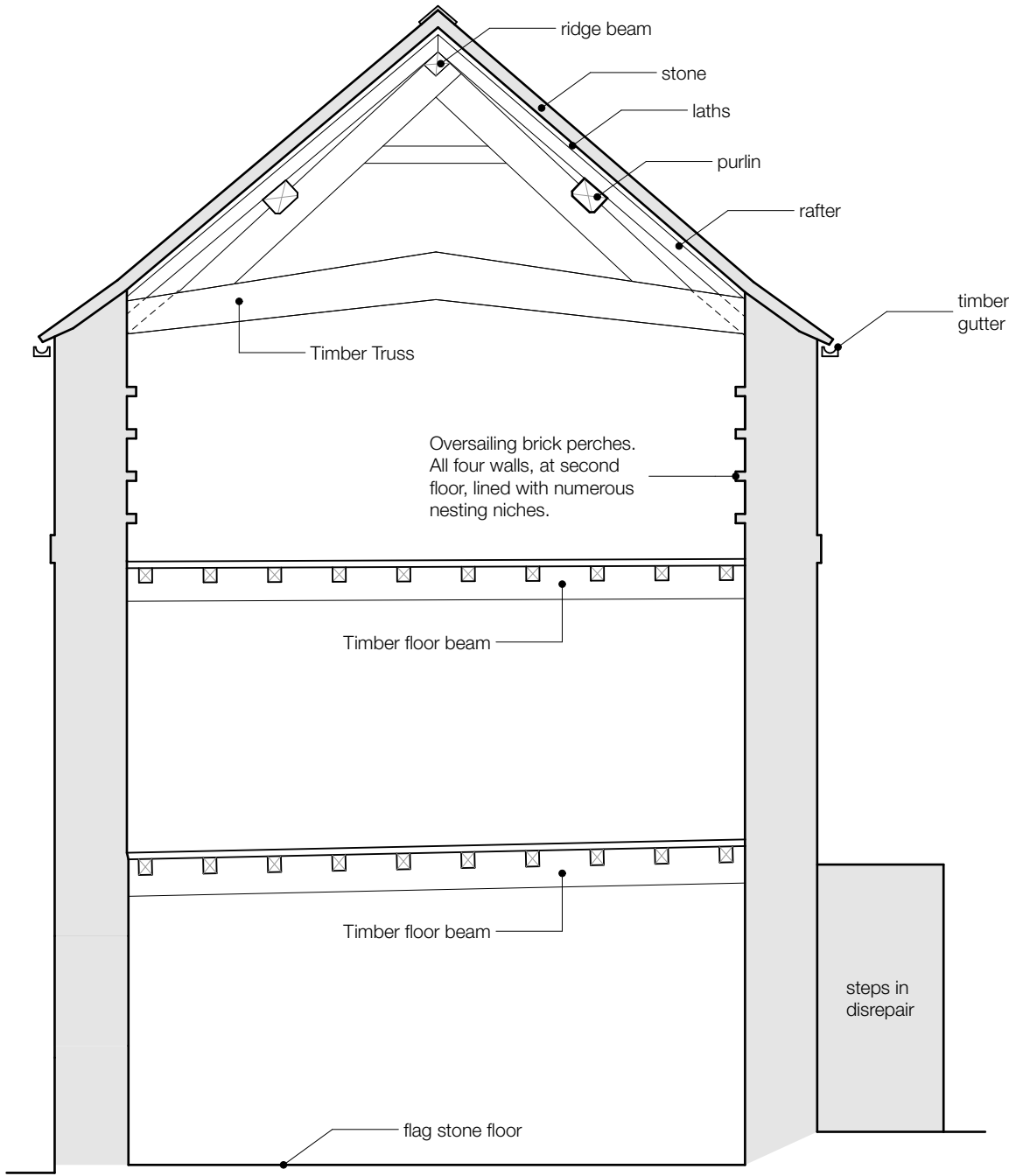
Section A (Existing)
