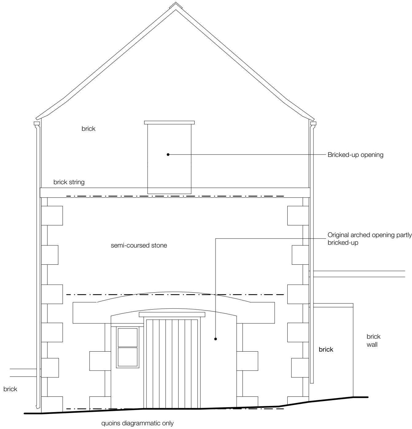
North Elevation (Existing)
