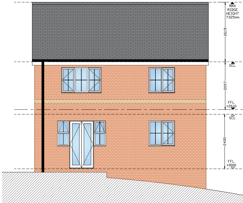
Elevation 03: Existing Rear Elevation
