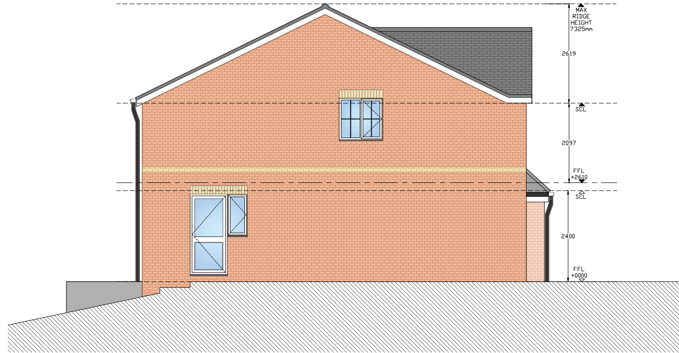
Elevation 02: Existing Side Elevation
