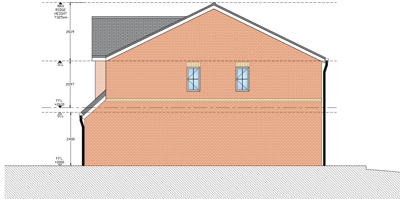
Elevation 04: Existing Side Elevation
