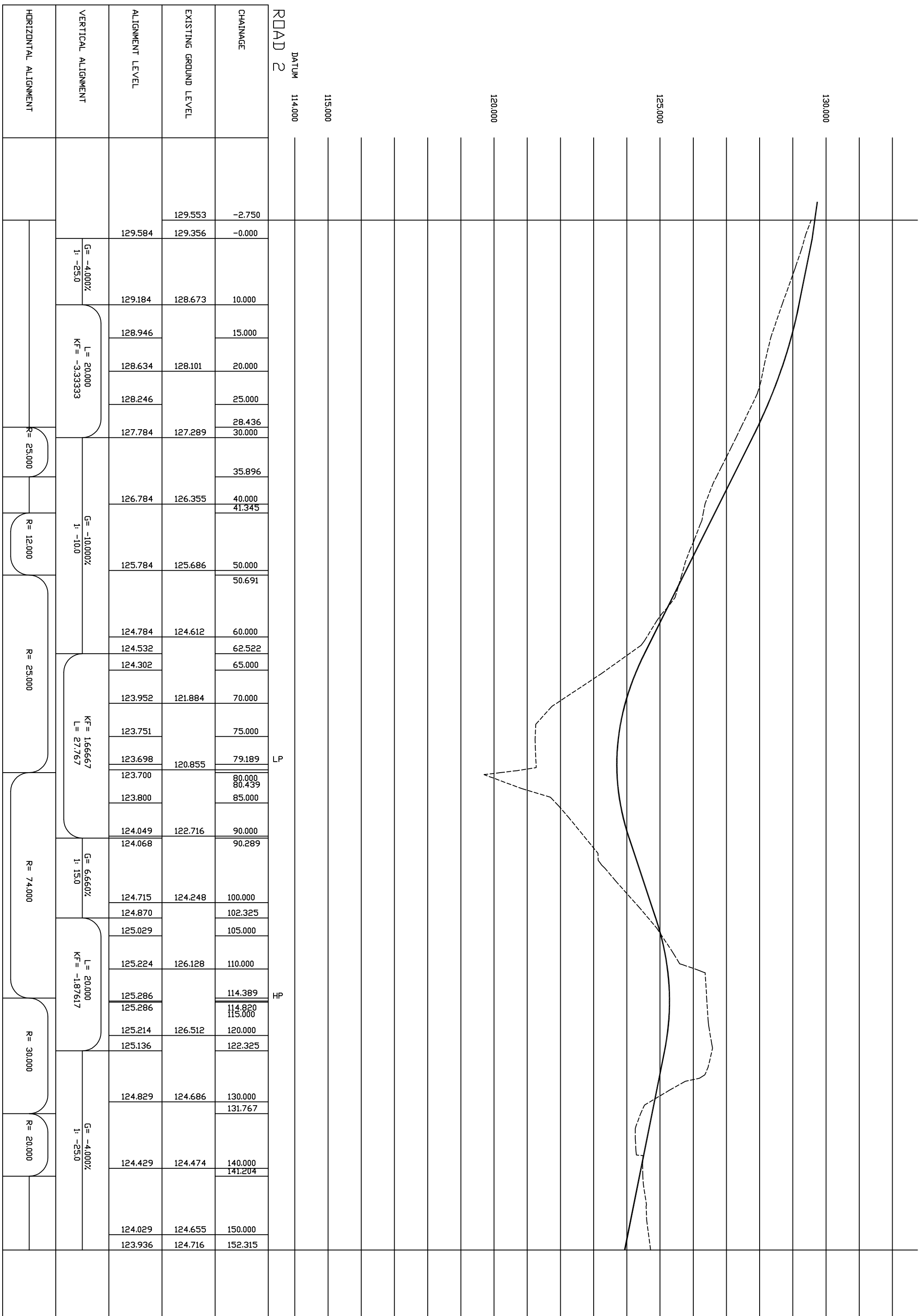
Road Longsection Scale 1:500 Hor 1:100 Ver
