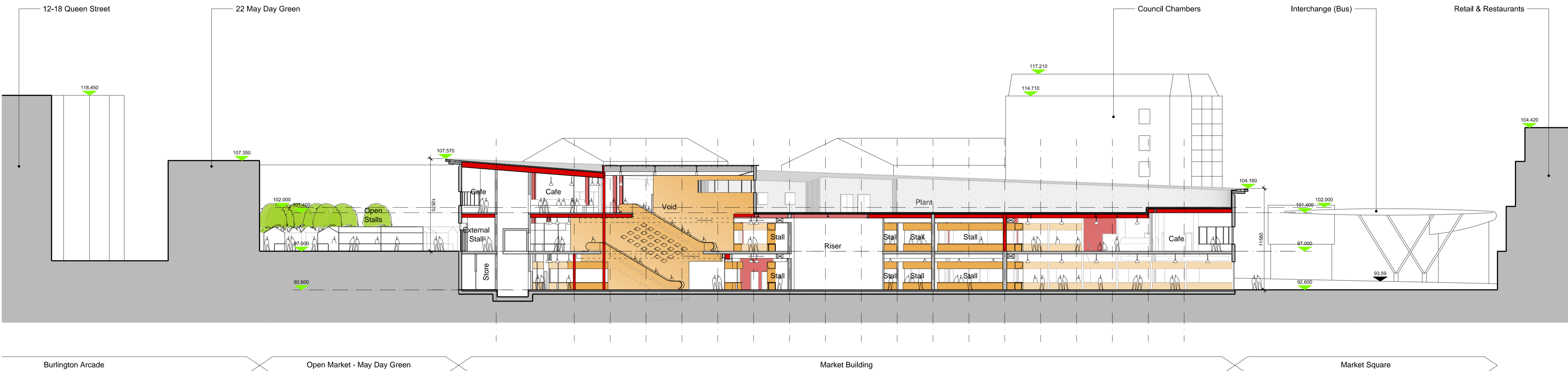
Market Section (03) 1:250
