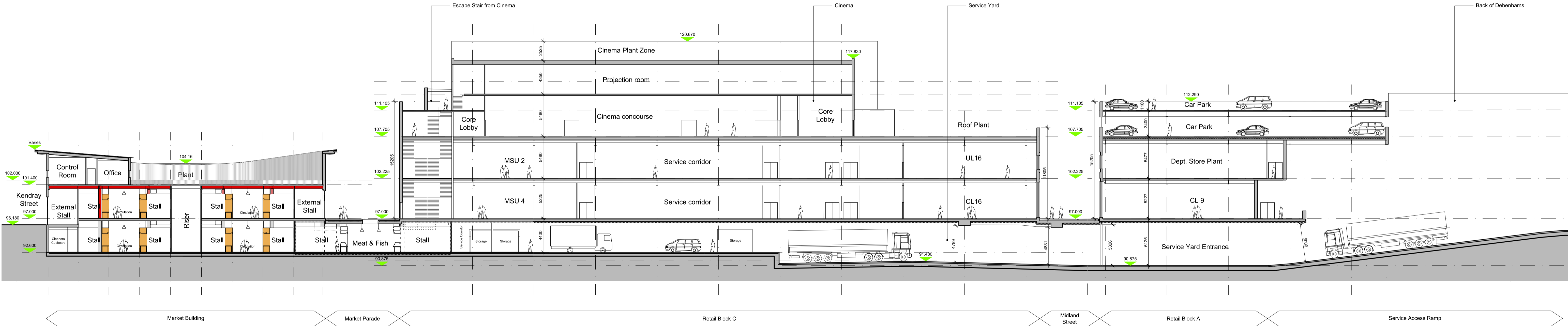
Market, Retail & Cinema Section (04) 1:250
