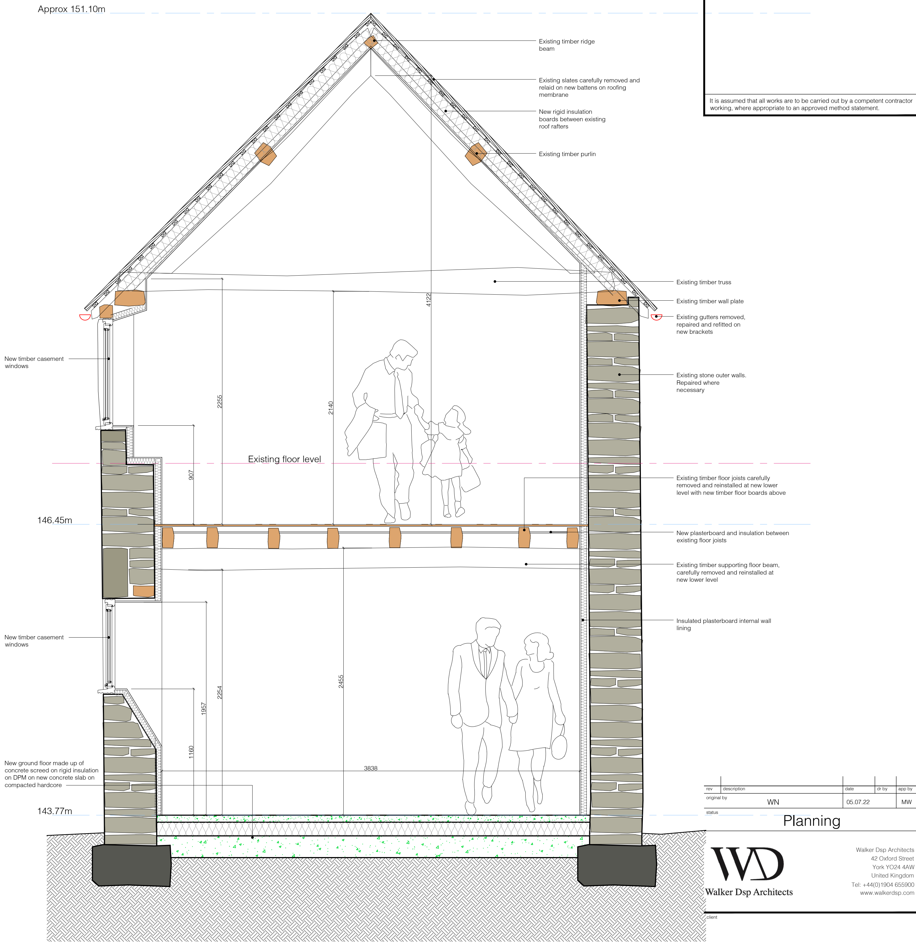
Barn 3 Proposed section AA
