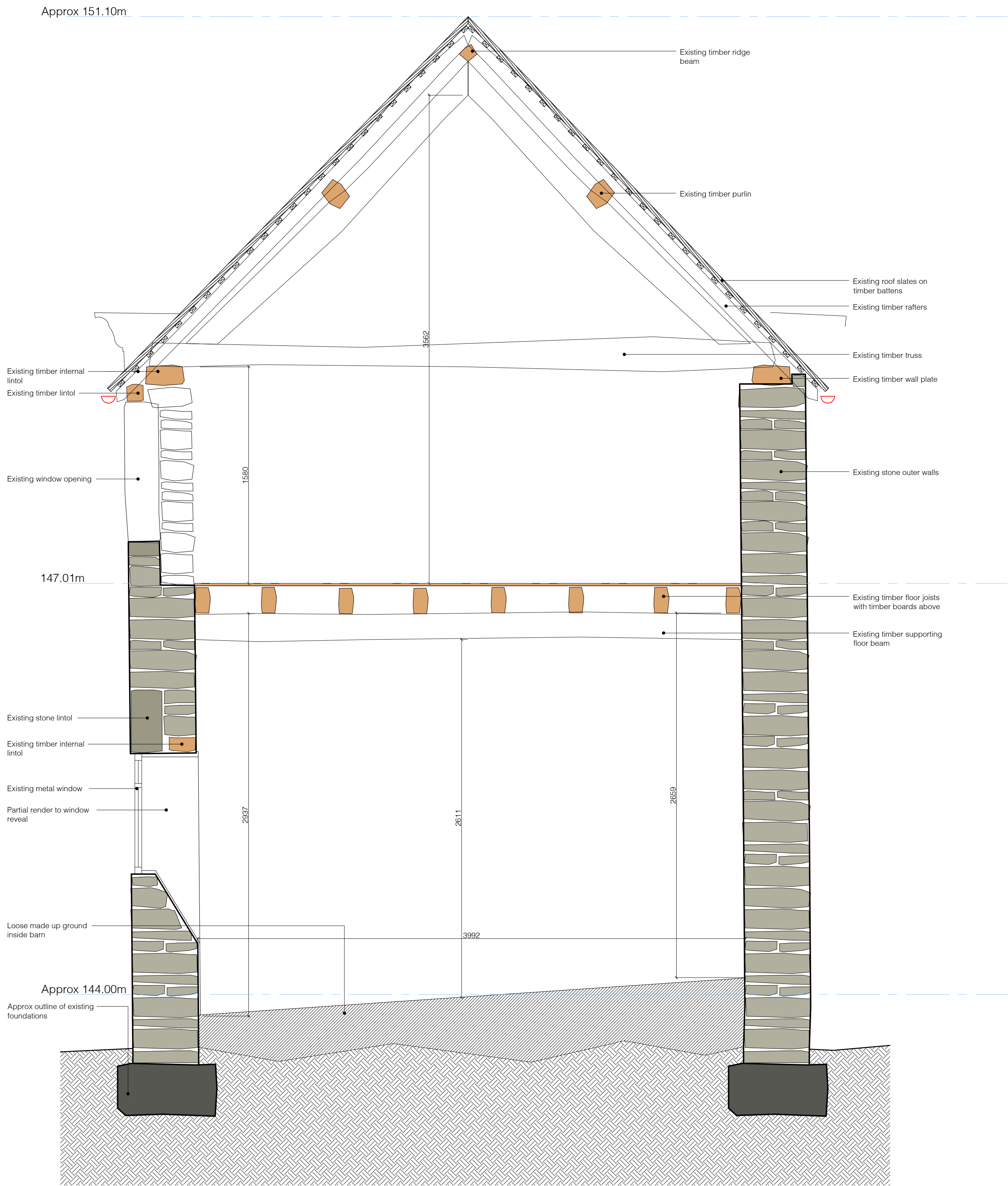
Barn 3 Existing section AA
