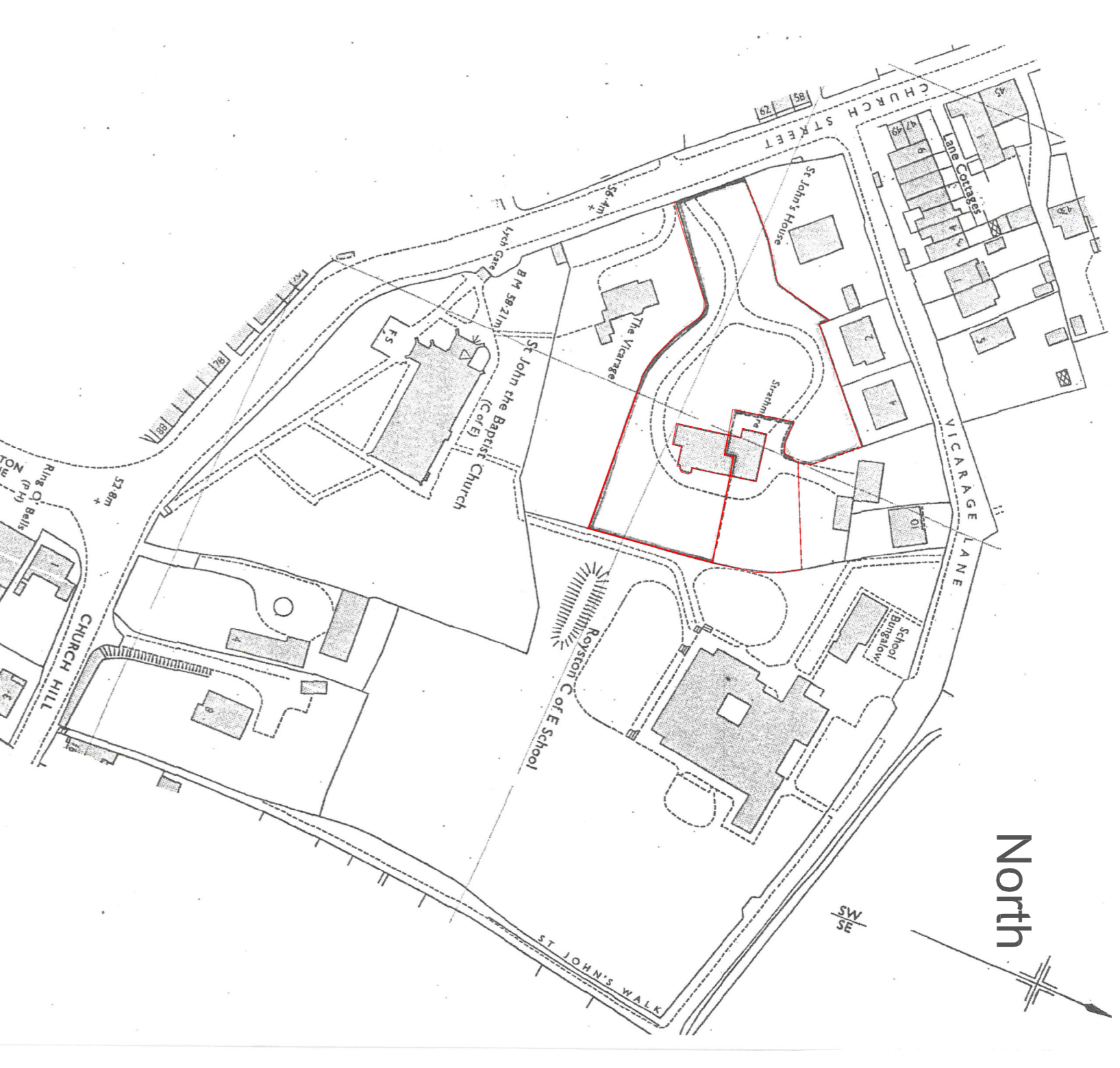
SITE LOCATION PLAN @ 1:1000
