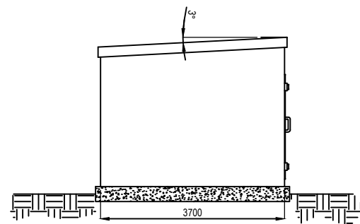
VIEW ON ARROW 'B'
