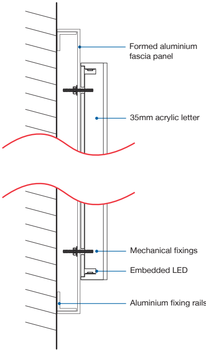
Section through - 1:5
