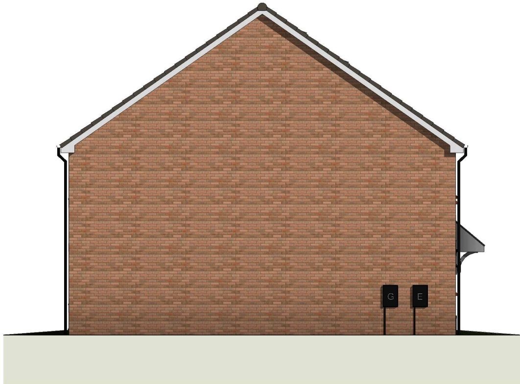
2 Gable Elevation 1 : 100
