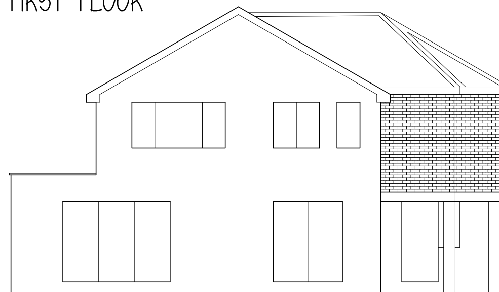
REAR ELEVATION
