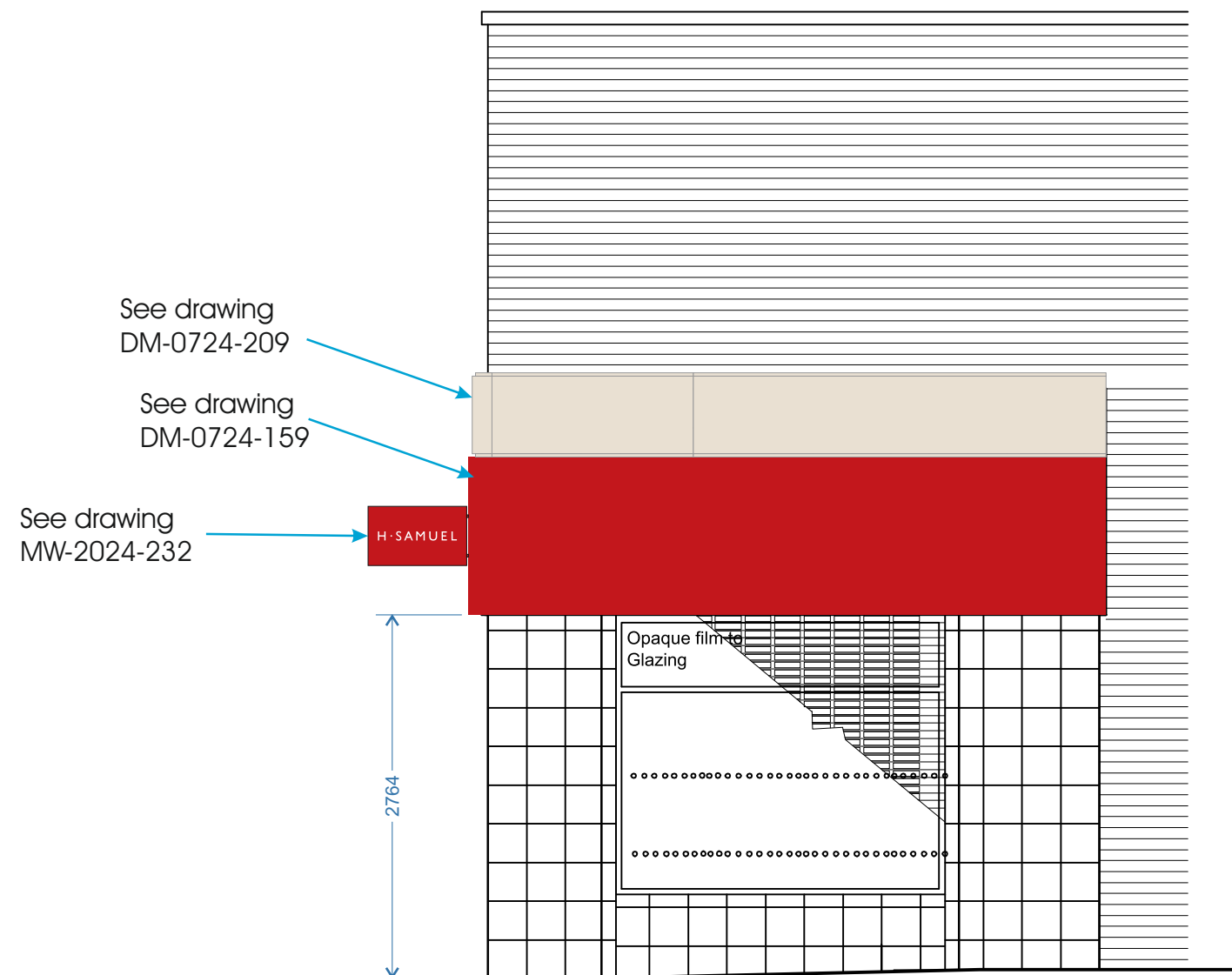
EXTERNAL ELEVATION B 1:50 scale
