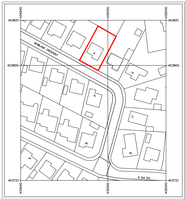
LOCATION PLAN 1:1250
