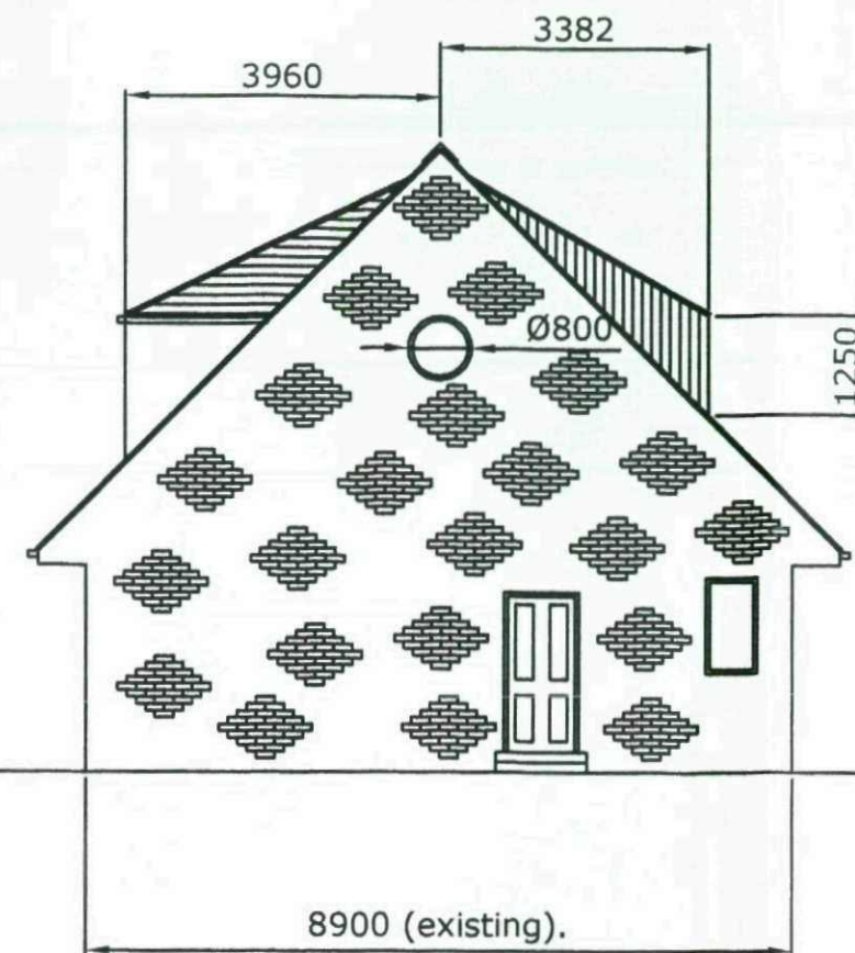
EAST ELEVATION.
