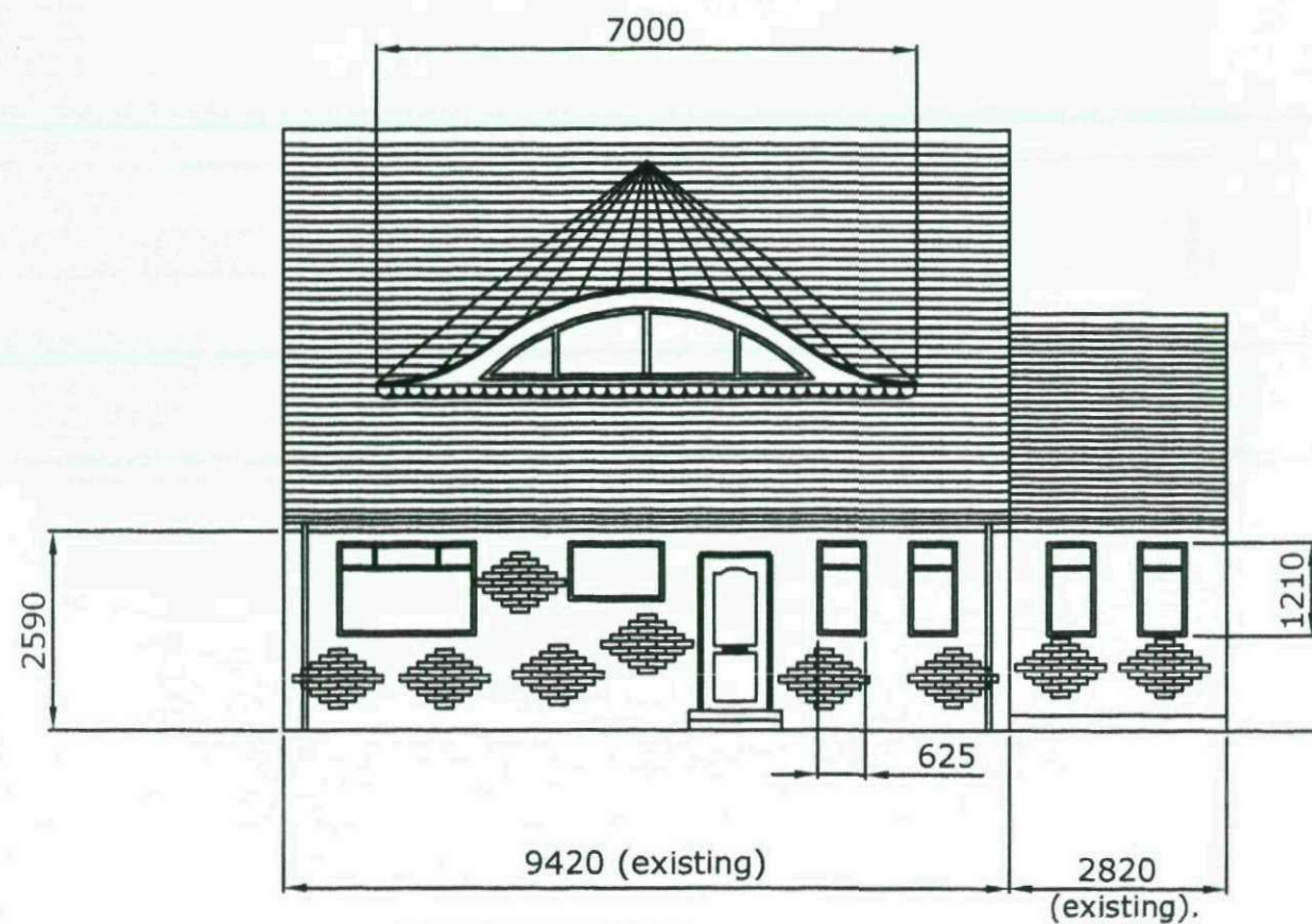
FRONT ELEVATION.
