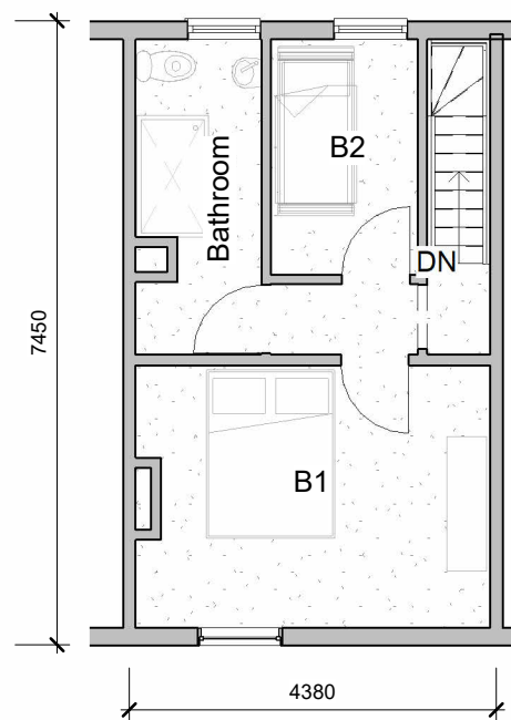
1st Floor Plan 1 : 100
