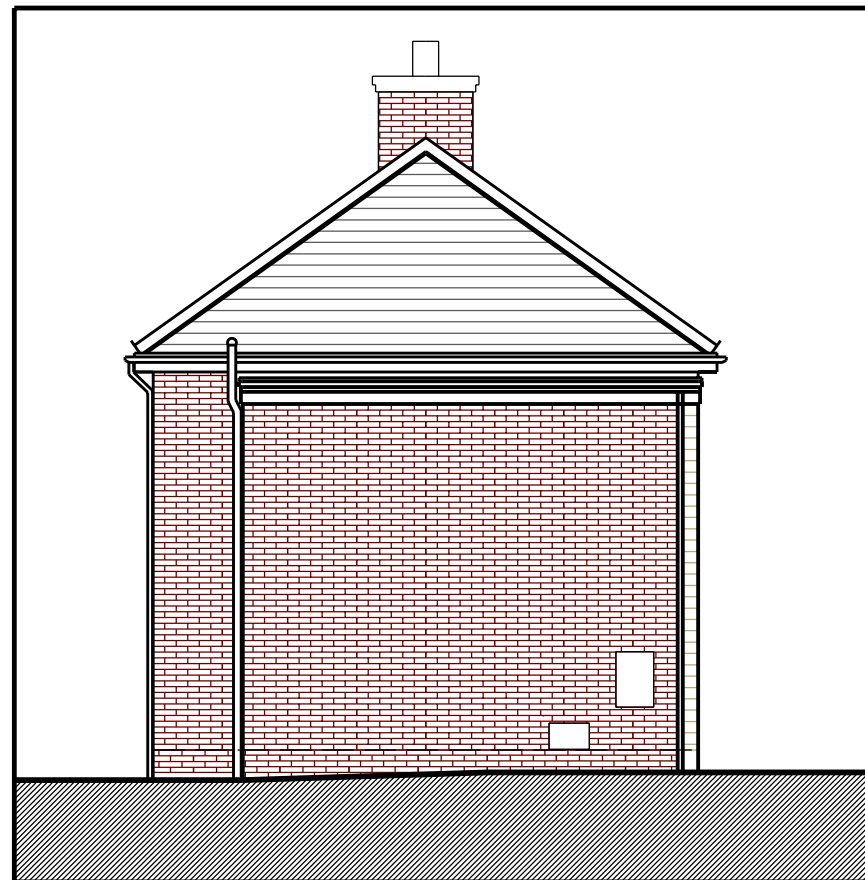
West Elevation
