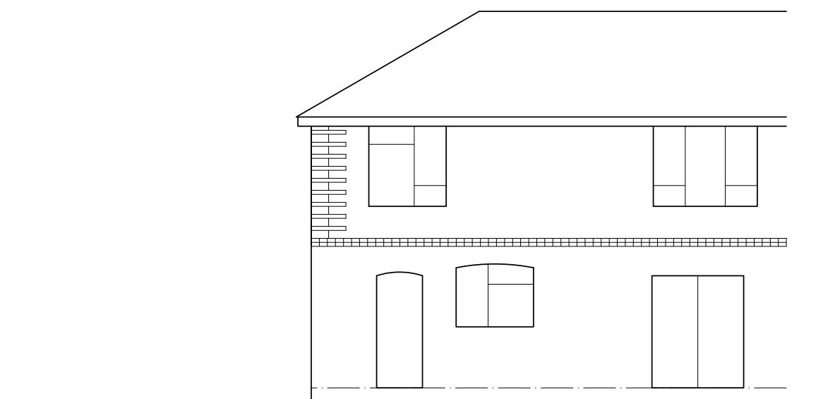
REAR ELEVATION
