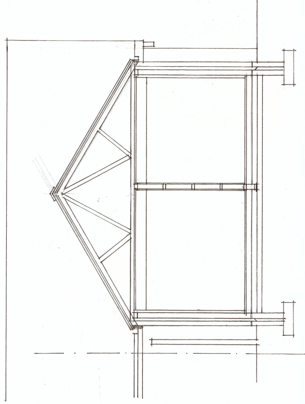
SECTION AA 1:50
