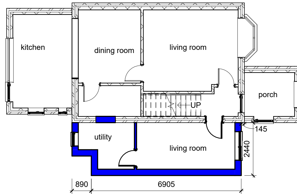
2 Ground Floor Proposed 1 : 100
