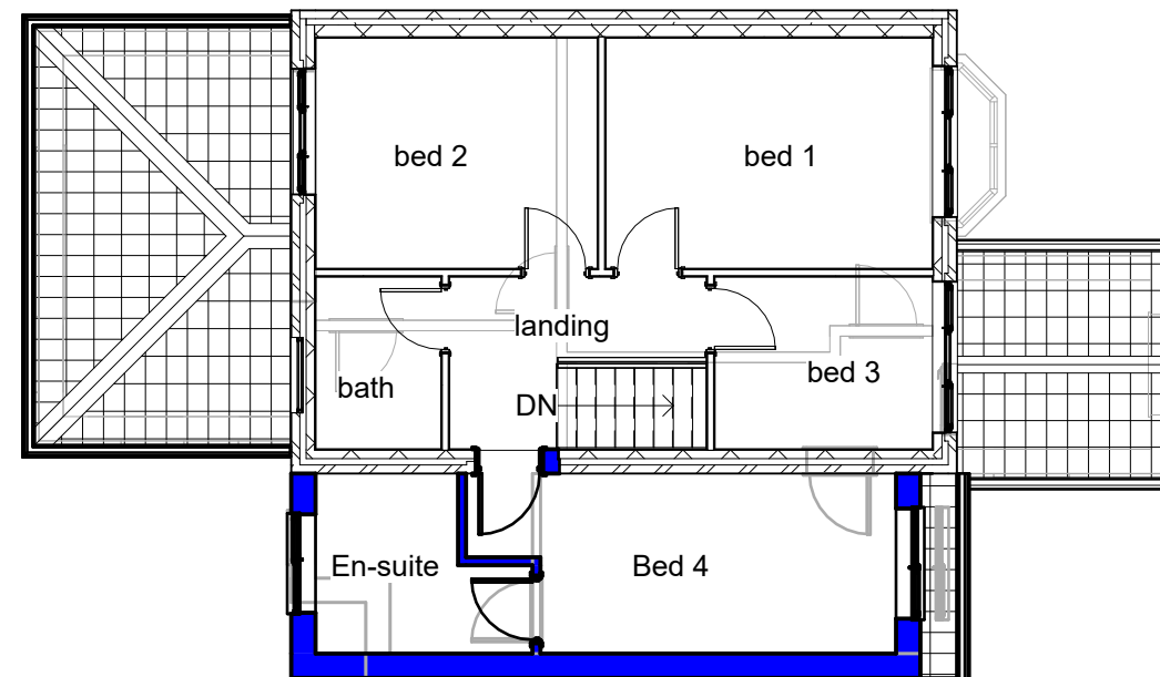
4 First Floor Proposed 1 : 100
