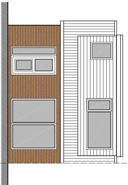
PROPOSED FRONT ELEVATION SCALE 1:100
