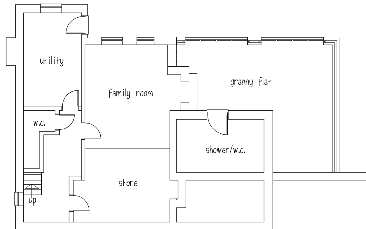
BASEMENT
