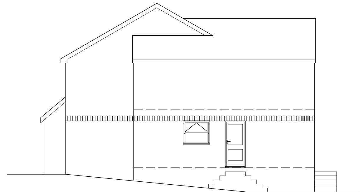
SIDE ELEVATION
