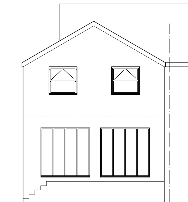
REAR ELEVATION
