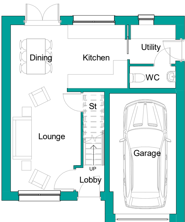
Ground Floor G.A. 1 : 100
