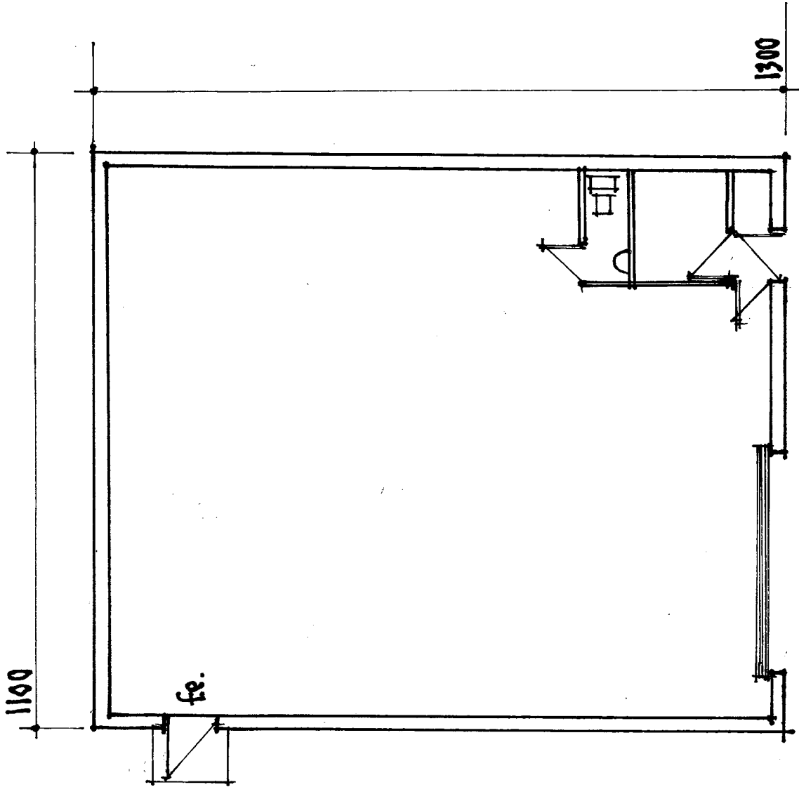
LAYOUT PLAN
