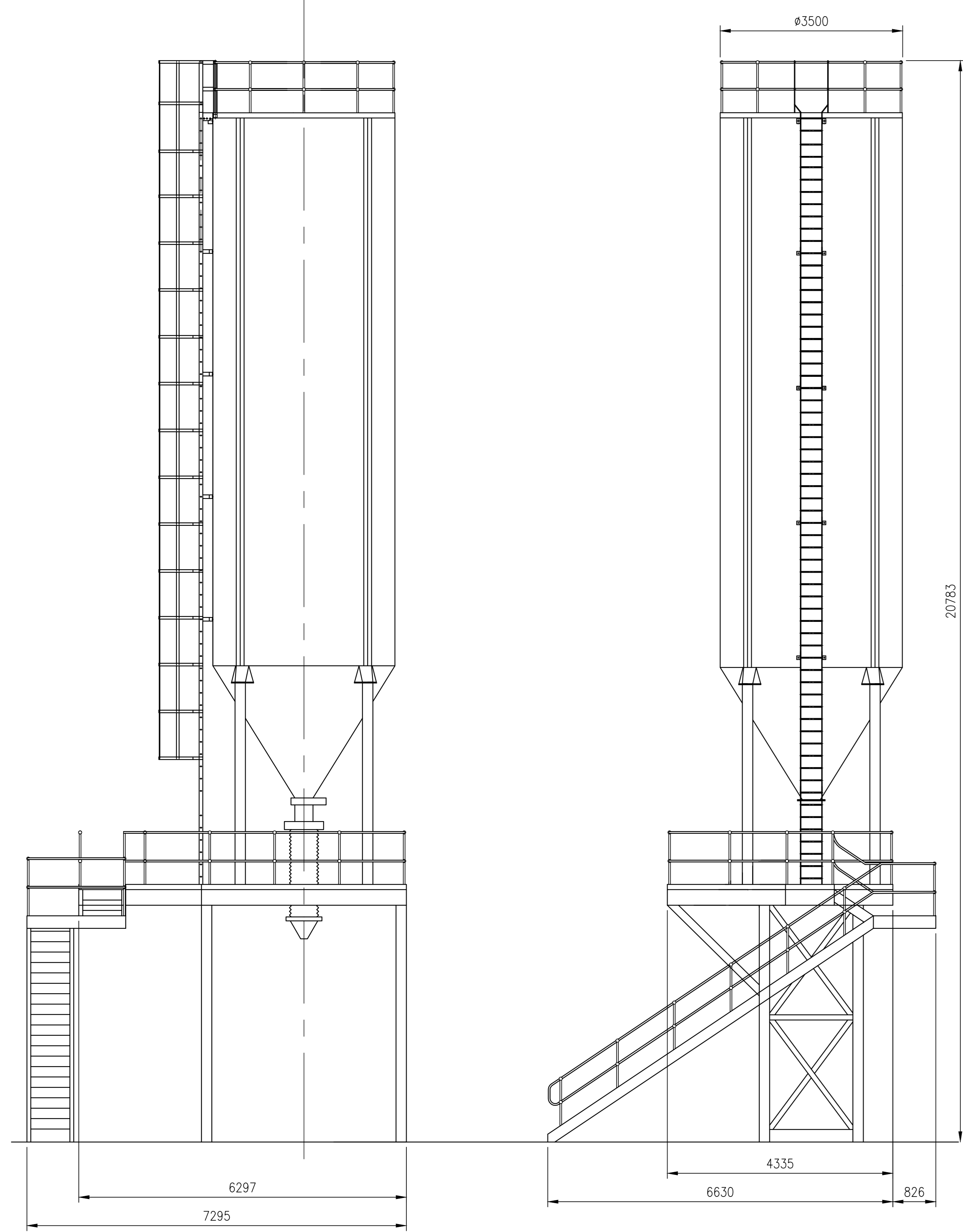
PROPOSED SILO SCALE ~ 1:50 @ A0
