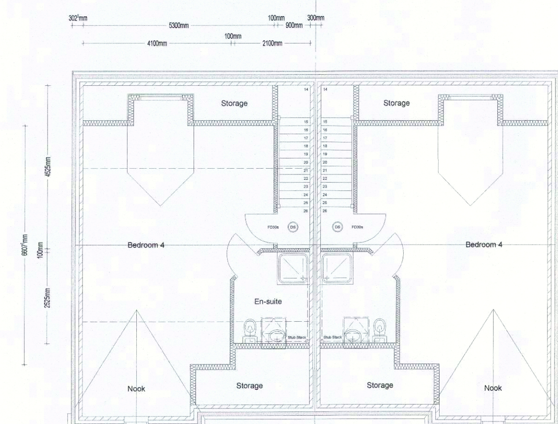
Second Floor Layout
