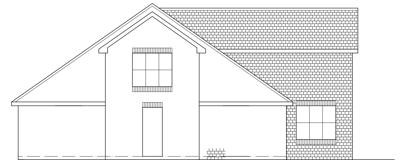
REAR ELEVATION (GRANGE LANE)
