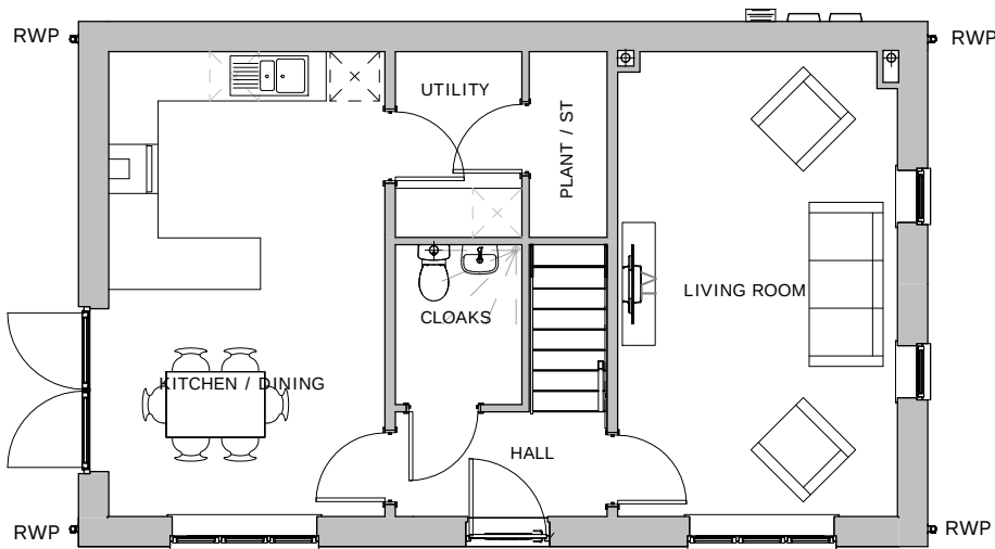
Ground Floor 1 : 100
