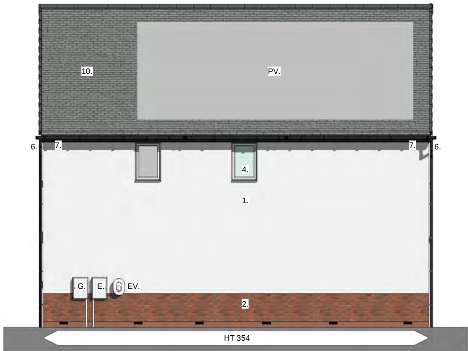
Side Elevation 1 : 100
