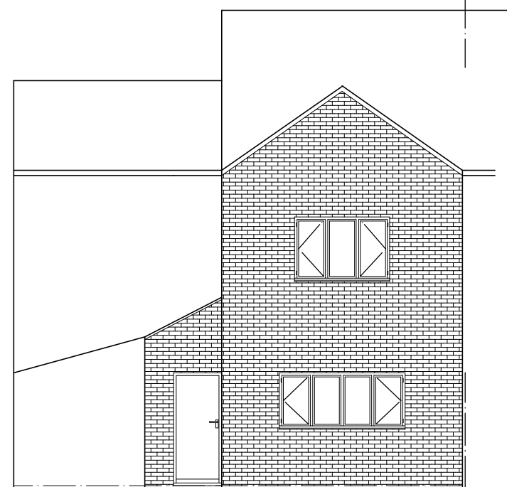
REAR ELEVATION
