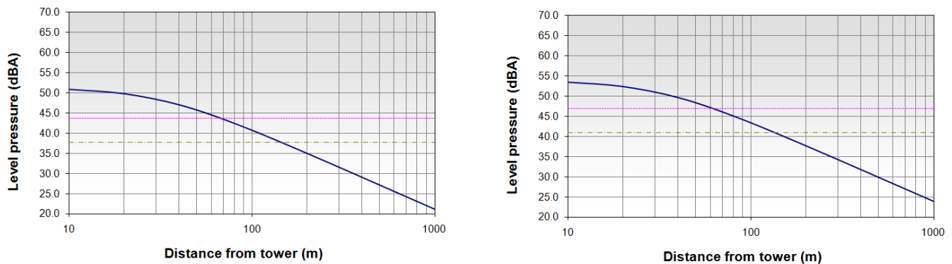
Figure 1. Sound level as a function of distance for the E- and G-Series turbines
