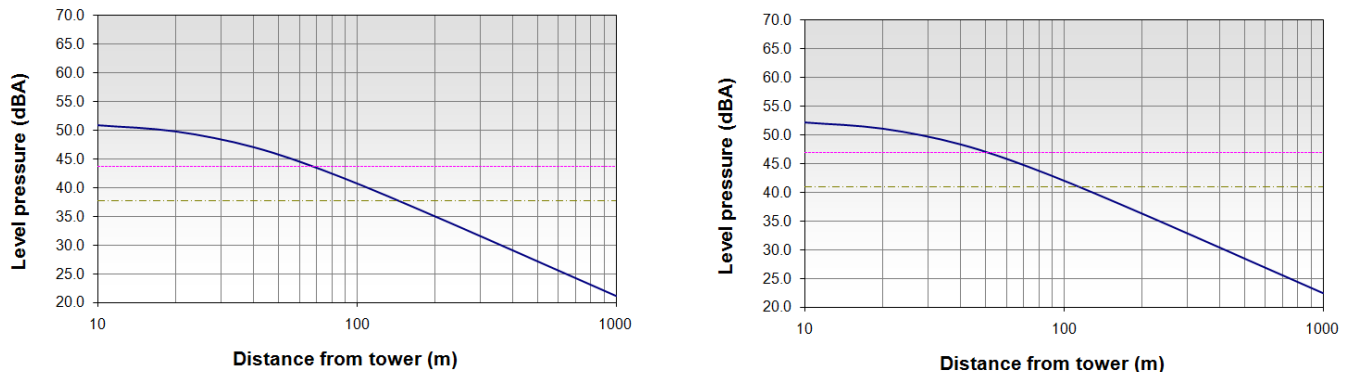
Figure 2. Sound level as a function of distance for the S-Series turbines
