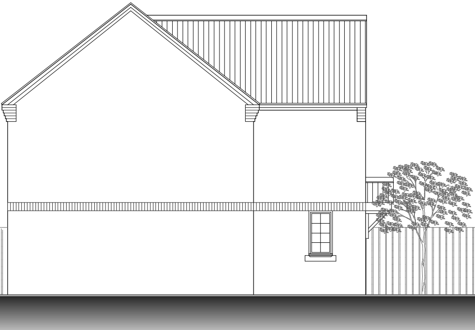
Side Elevation
