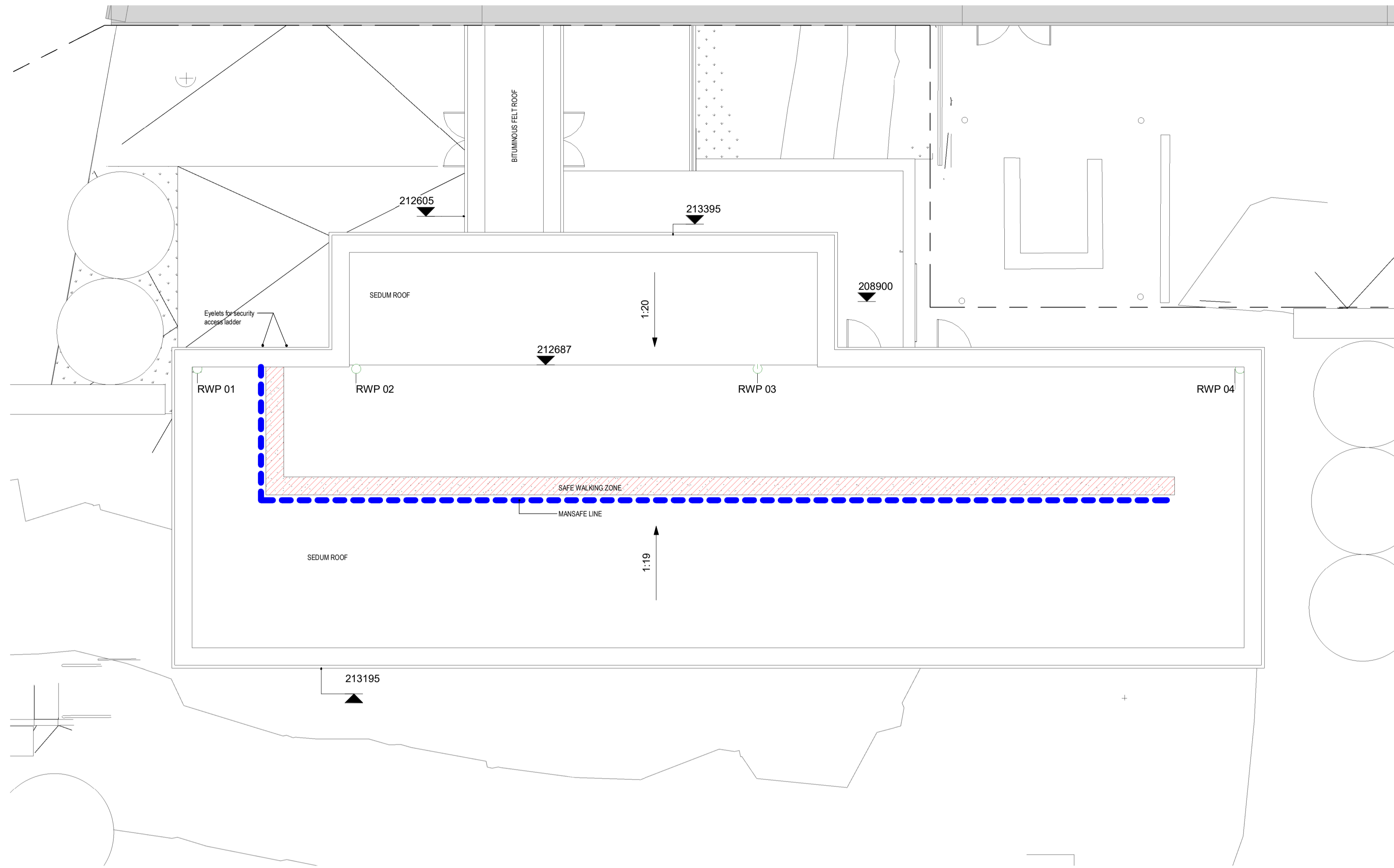
1 Roof Plan 1:100 Ref Sheet: 0301
