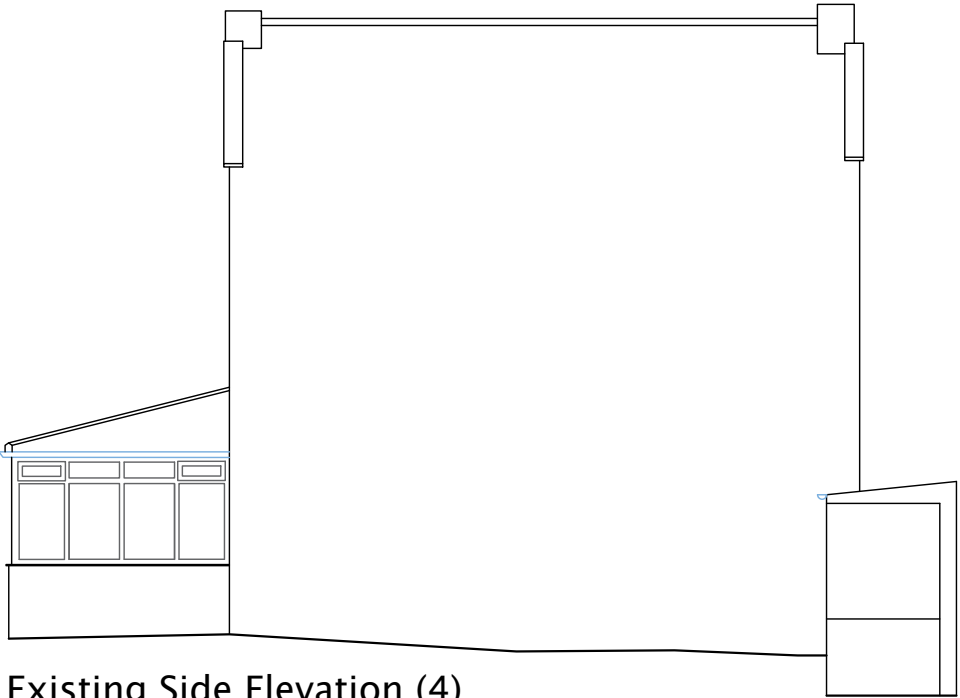
Existing Side Elevation (4)
