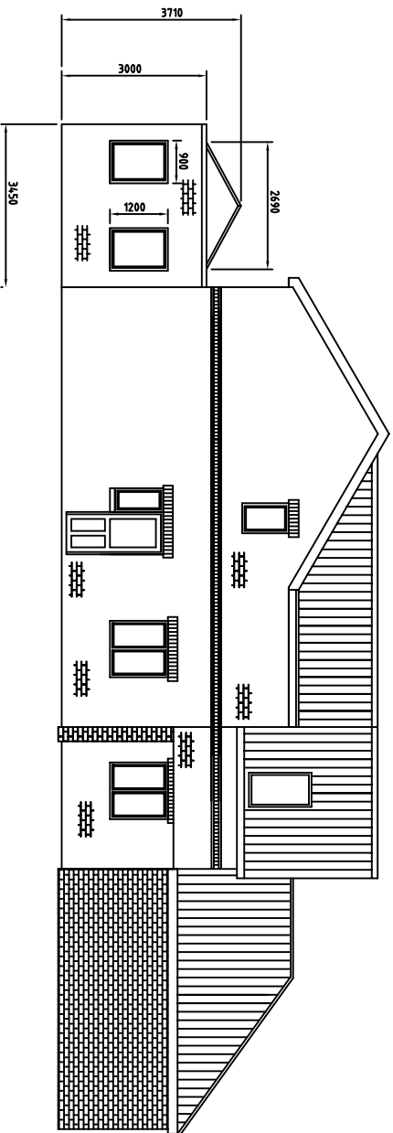
side elevation
