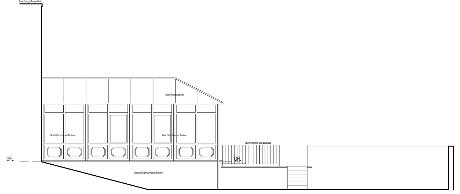
Rear NW Elevation (A) as Existing
