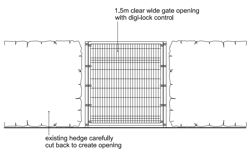
PROPOSED GATE / FENCE DETAIL 1:50
