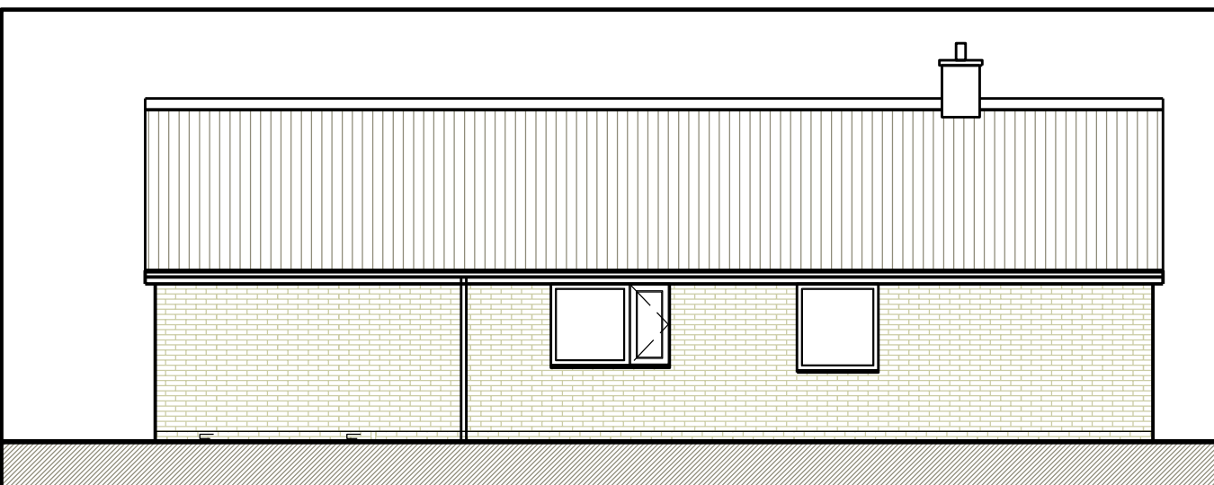
South Elevation
