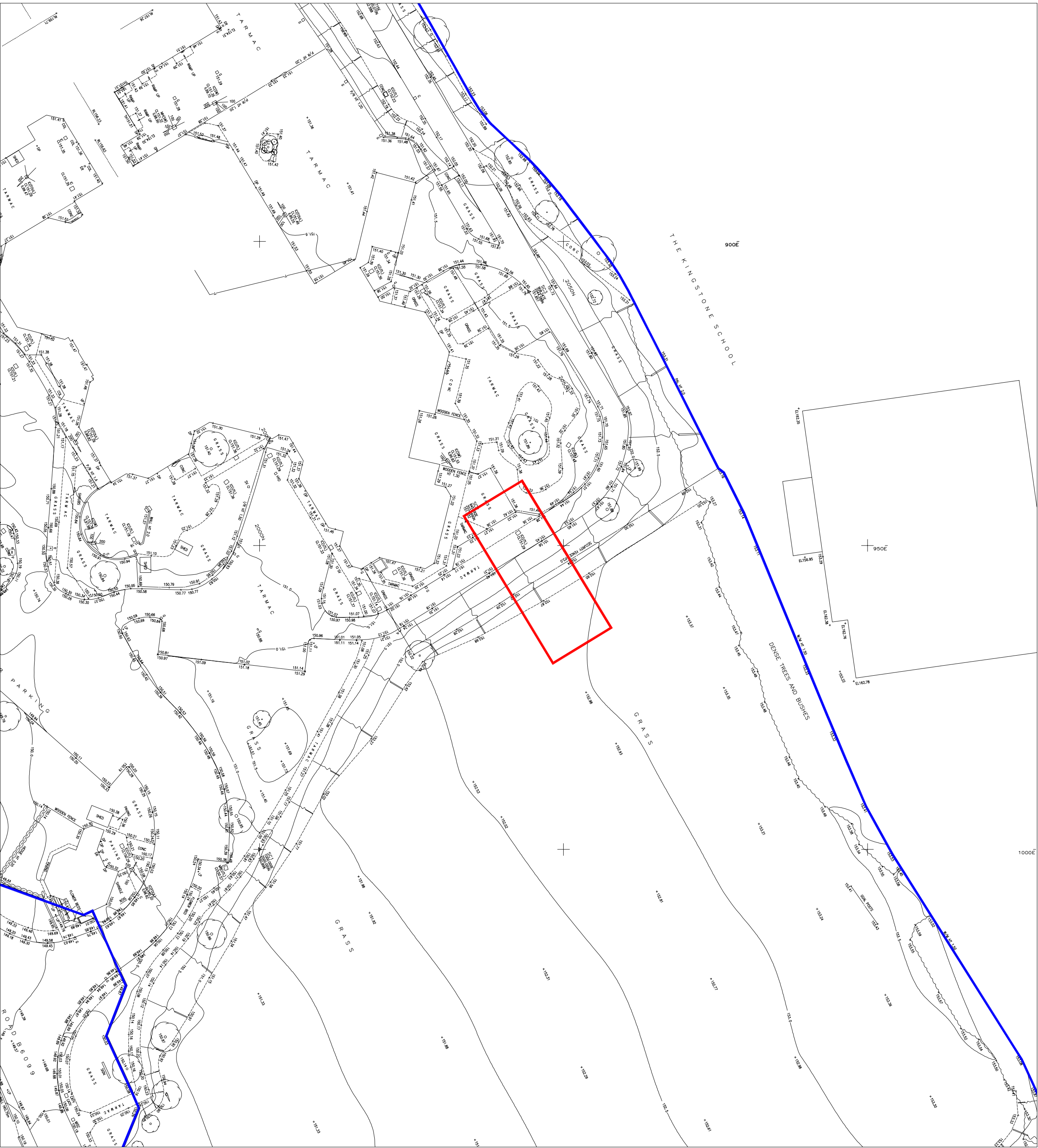
INSET A - Partial Site Topographical Survey - 1:500
