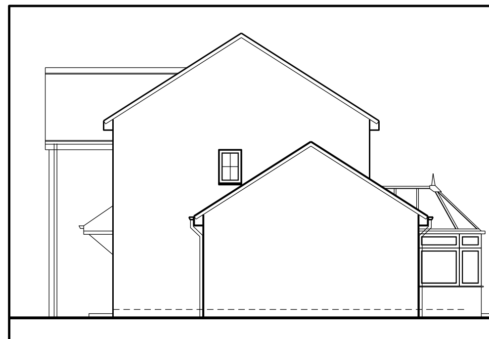
East Elevation - Existing
