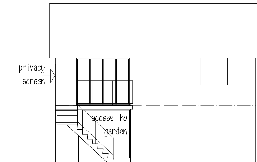
REAR ELEVATION
