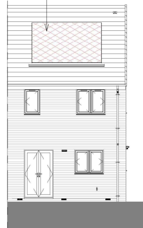
Rear Elevation.
