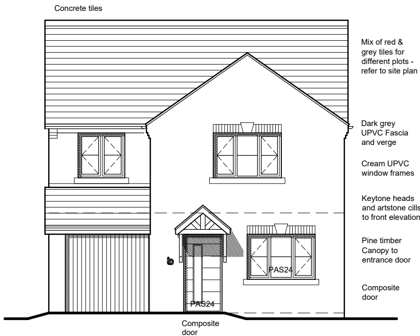
FRONT ELEVATION
