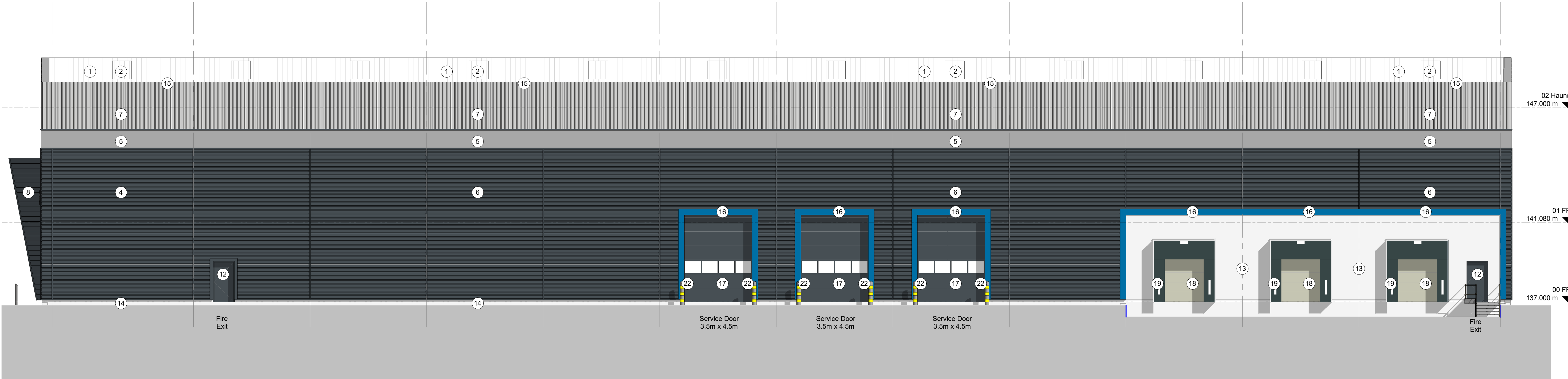
Service Yard Elevation 1 : 100
