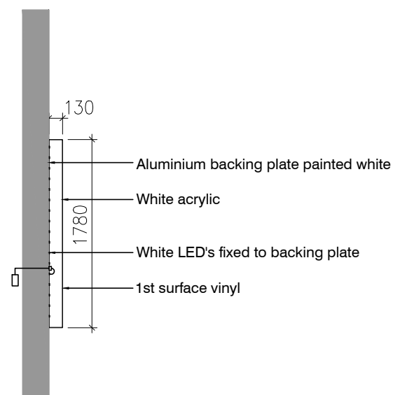
SECTION
