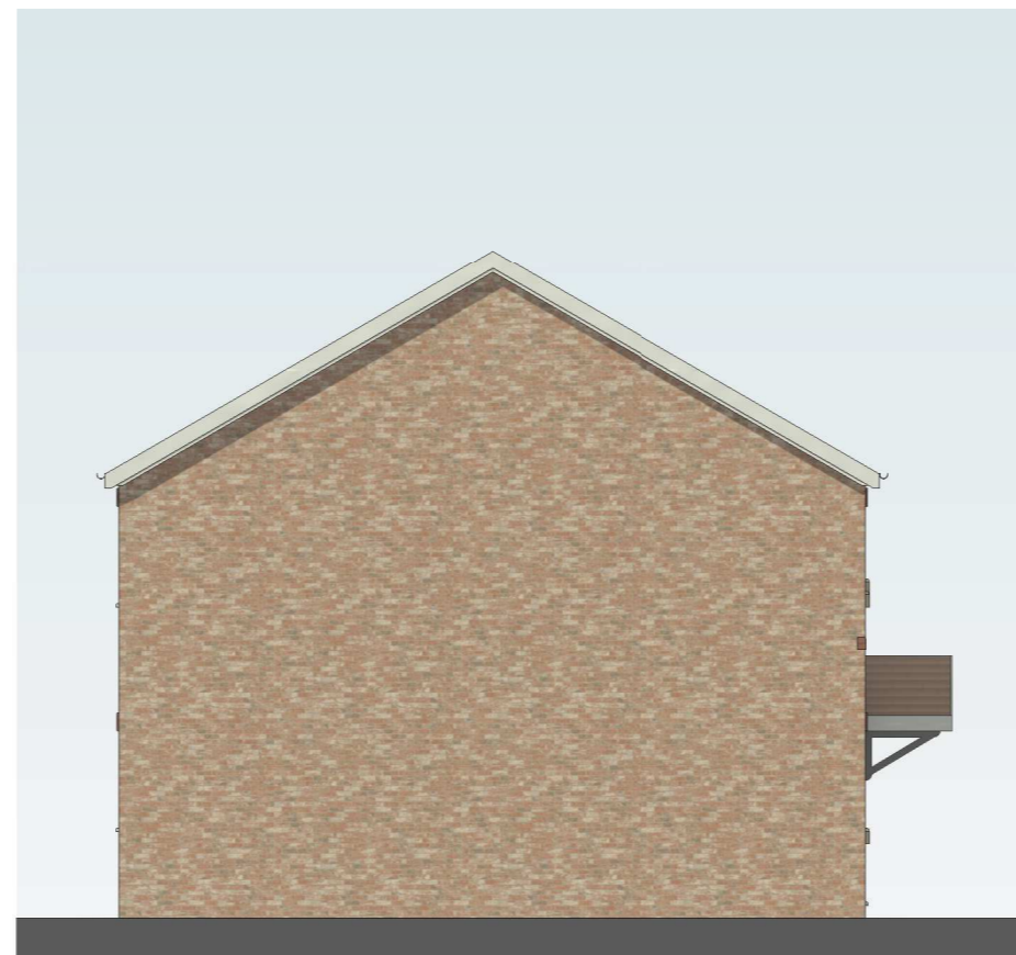
5 | HTA SIDE_Elevation 1 : 100
