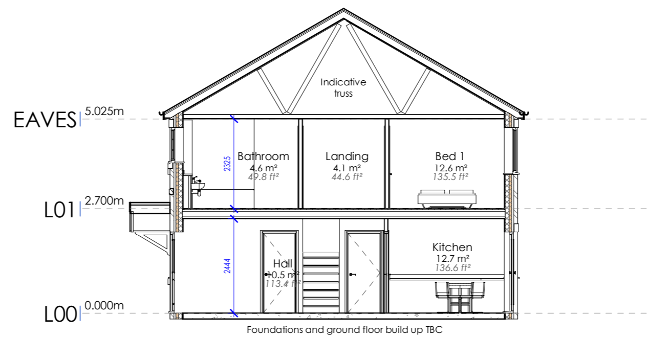
7 | HTA Section 1 : 100
