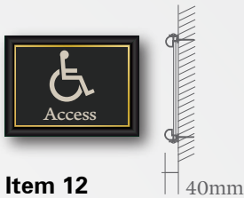
Item 12 1no Small bullnose access sign. Size: 400mm x 300mm Scale: 1:20
