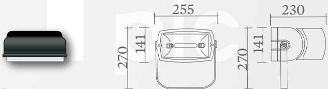
Item 15 4no replacement LED flood lights. Scale: 1:20
