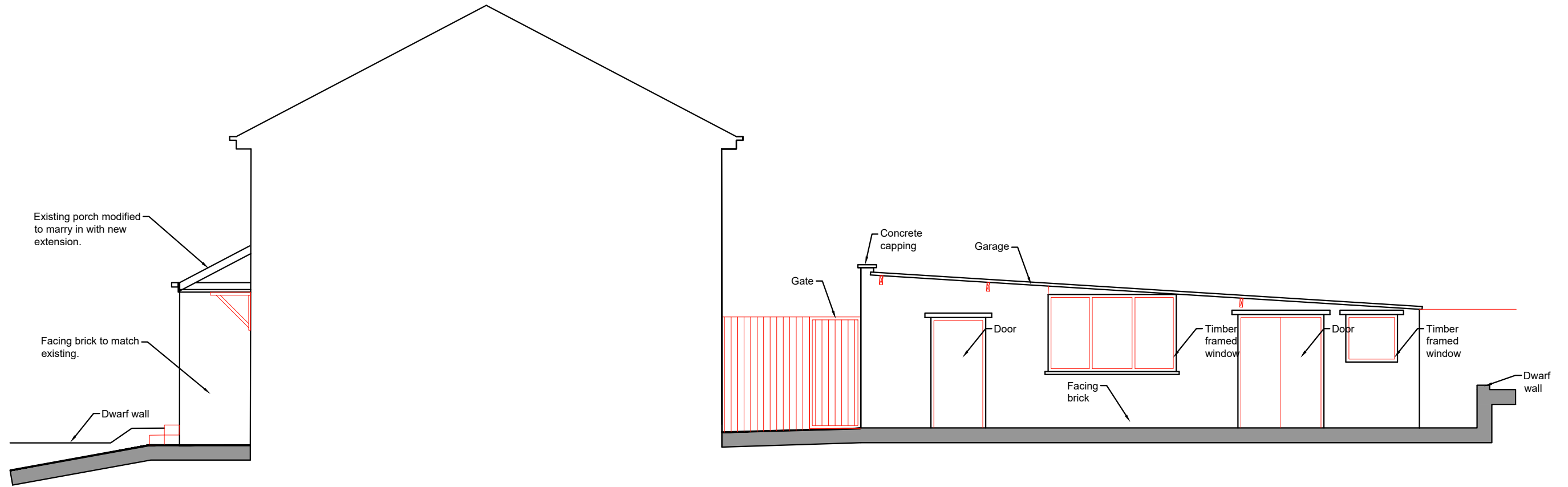
Proposed Side Elevation neighbours side. Viewed from no 10.
