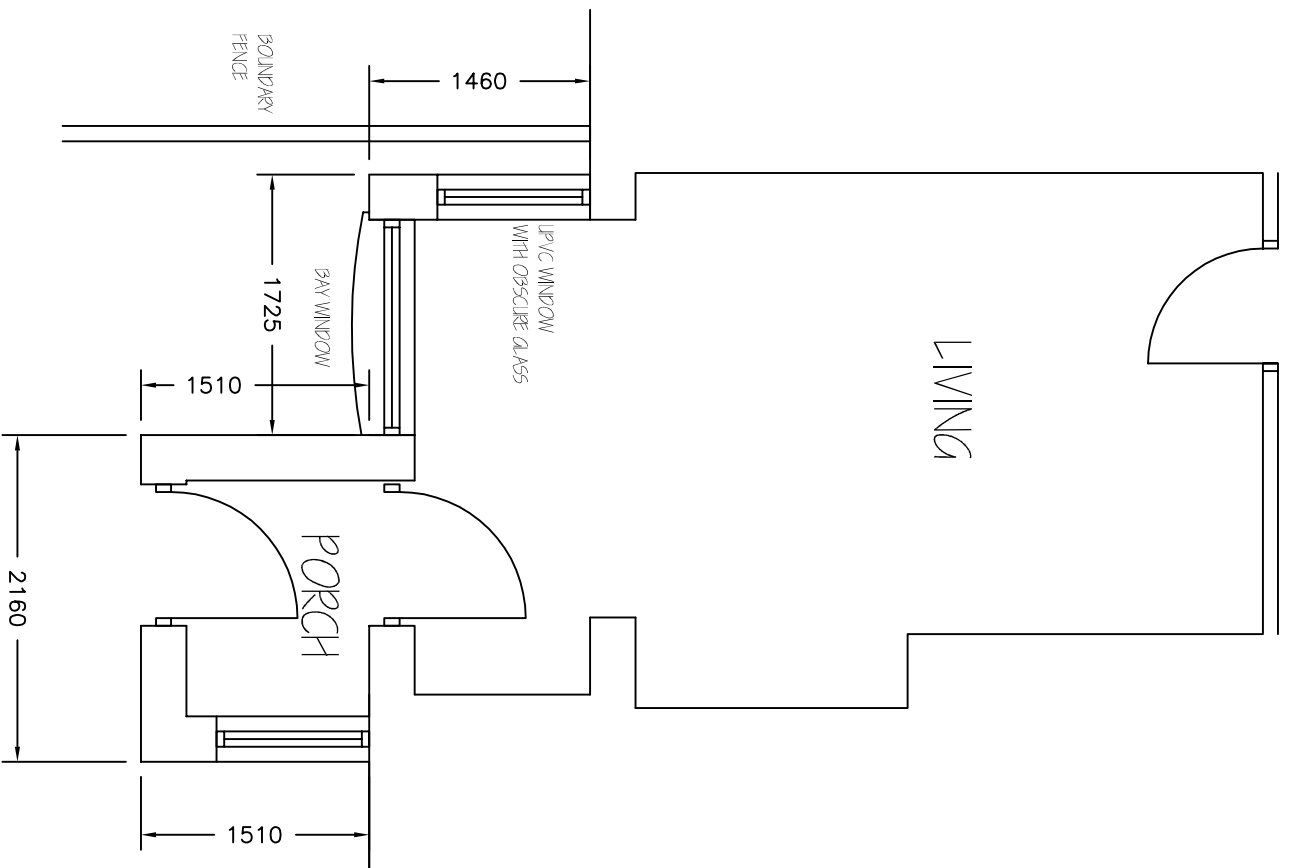
PROPOSED PLAN 1:50
