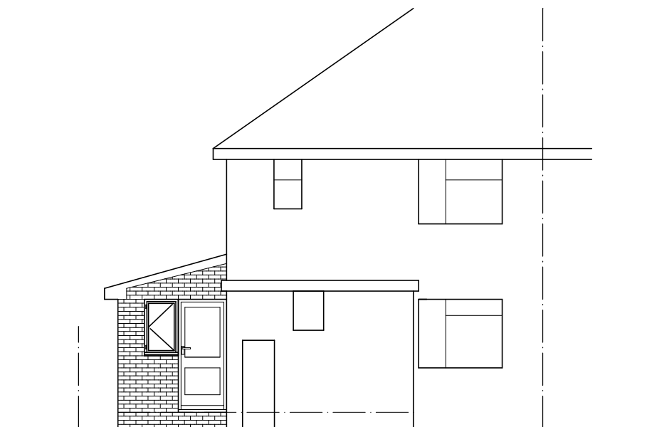
REAR ELEVATION
